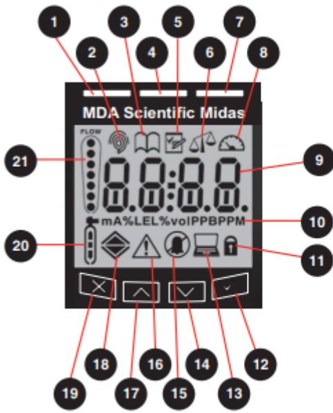
Diagram 2-3. Midas® display module layout
