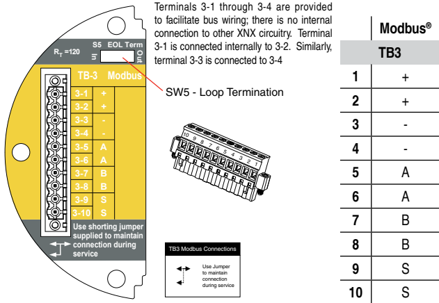
Figure 1. XNX Modbus® Option Board Terminal Block and Jumper Switch
